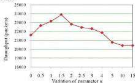
Figure 5. Network throughput
